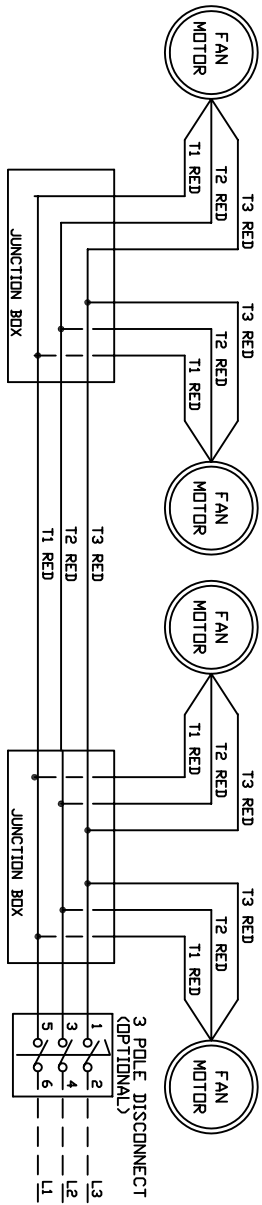
4 FAN WIRING DIAGRAM W/ OPTIONAL DISCONNECT
